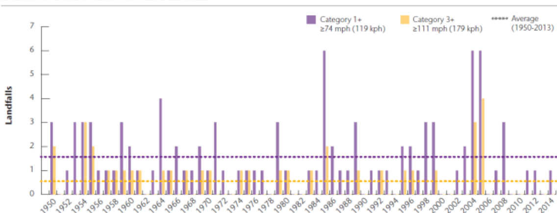
Exhibit 80: United States Hurricane Landfalls
