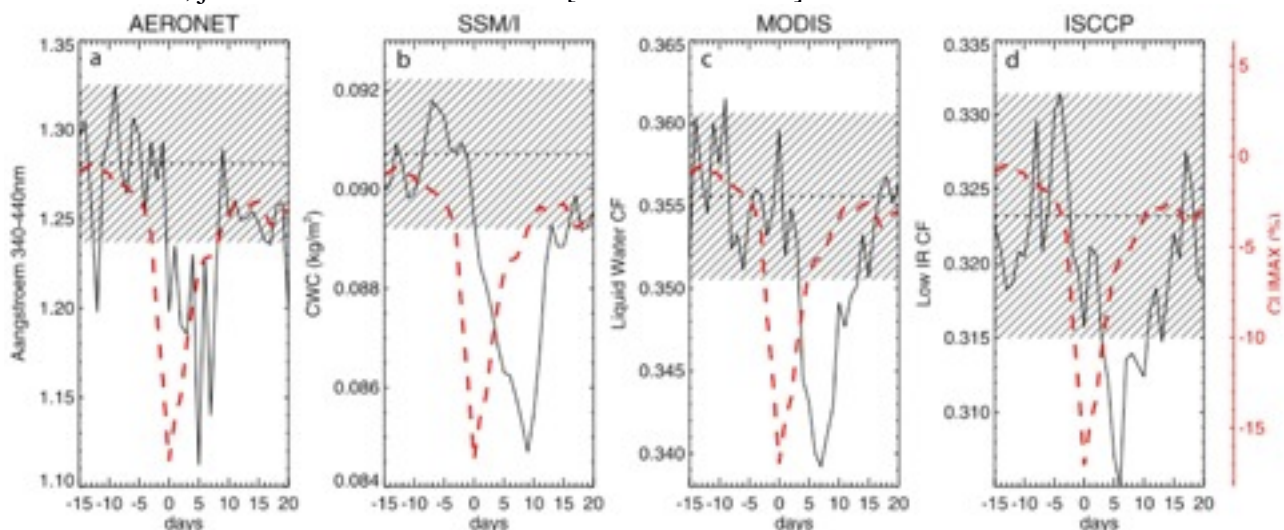
Figure 18 The evolution of [b] cloud water content [SSM/I], c] liquid water cloud fraction [MODIS], and d] low IR-detected clouds [ISCCP] is here averaged for the five strongest Forbush decreases that their data sets have in common and is compared with a] the corresponding evolution of fine aerosol particles in the lower atmosphere [AERONET]. In a] each data point is the daily mean from about 40 AERONET stations world-wide, using stations with more than 20 measurements a day. Red curves show % changes in GCR neutron counts at Climax. The broken horizontal lines denote the mean for the first 15 days before the Forbush minimum, and the hatched zones show \pm 1\sigma for the data, estimated from the average variance of a large number of randomly chosen periods of 36 days of each of the four data sets. The effects on clouds and aerosols are not dominated by any single event among the 5 averaged.
