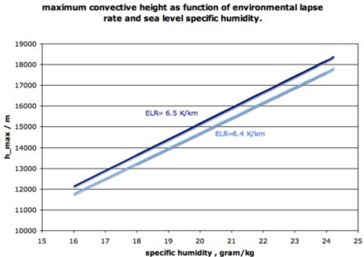
Figure 3 Maximum height of a tropical thunderstorm cloud as function of the sea level specific humidity and the environmental lapse rate.
