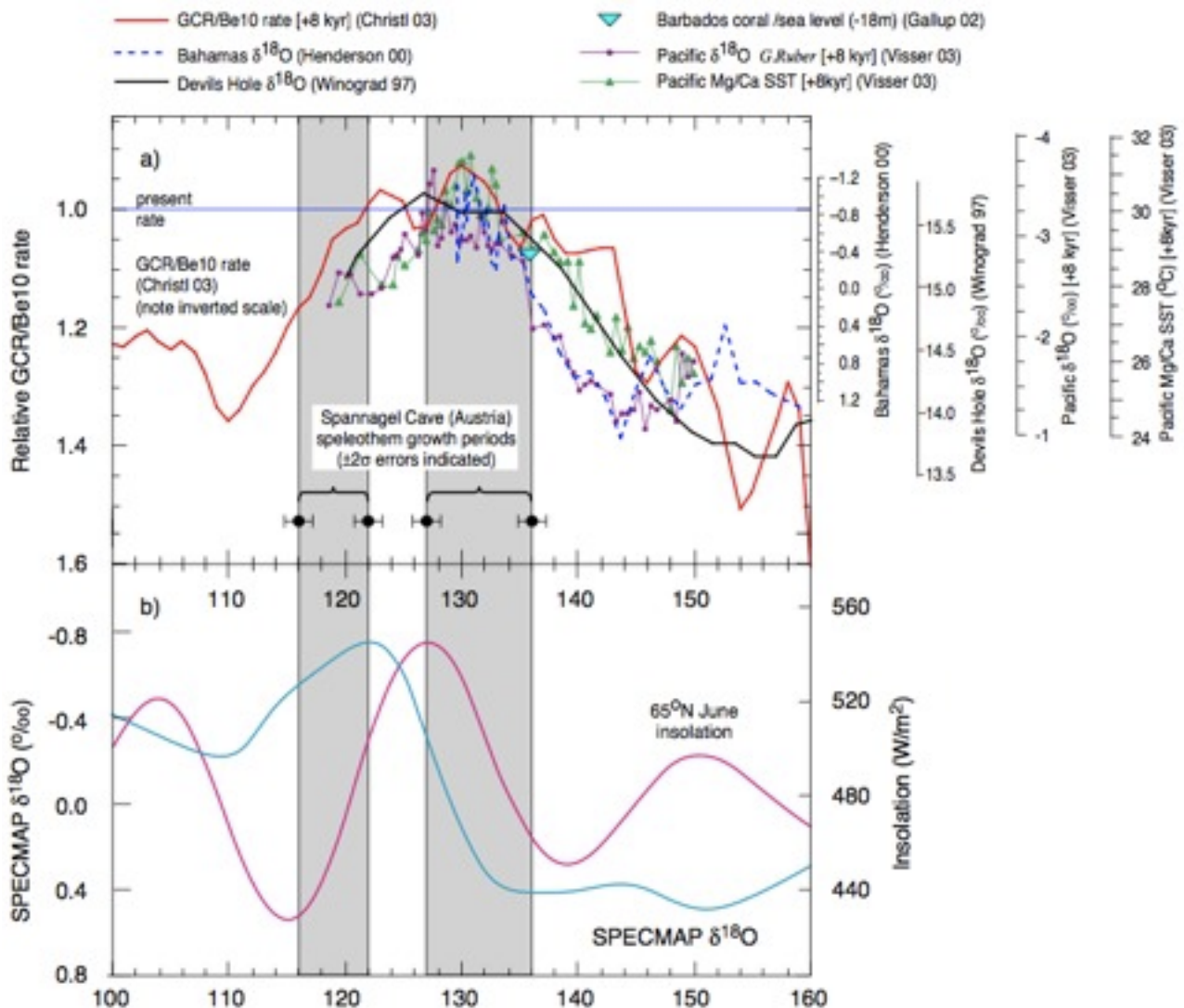
Figure 23 Timing of glacial Termination II, 130 kyr ago. a) The GCR rate together with the Bahamian \delta^{18}\text{O} record, the date when the Barbados sea level was within 18 m of its present value, the \delta^{18}\text{O} temperature record from Devils Hole cave, Nevada, and the Visser et al. measurements of the Indo-Pacific Ocean surface temperature and \delta^{18}\text{O} records. The GCR rate and the Visser et al. data are shifted earlier by 8 kyr in order to correct for estimated systematic errors in the SPECMAP timescale, on which they are based. The growth periods of stalagmite SPA 52 from Spannagel Cave, Austria, are indicated by grey bands and black points. b) The 65°N June insolation and the SPECMAP \delta^{18}\text{O} record.
